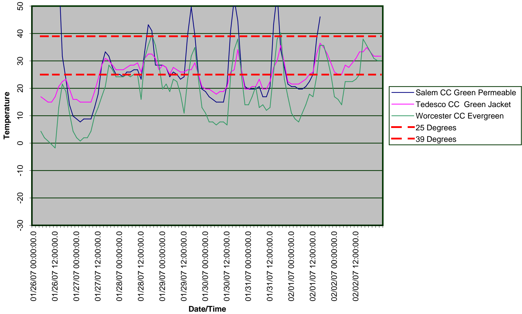
Below Cover Temps 1-26-07 to 2-2-07 (2 Hr. Readings)
