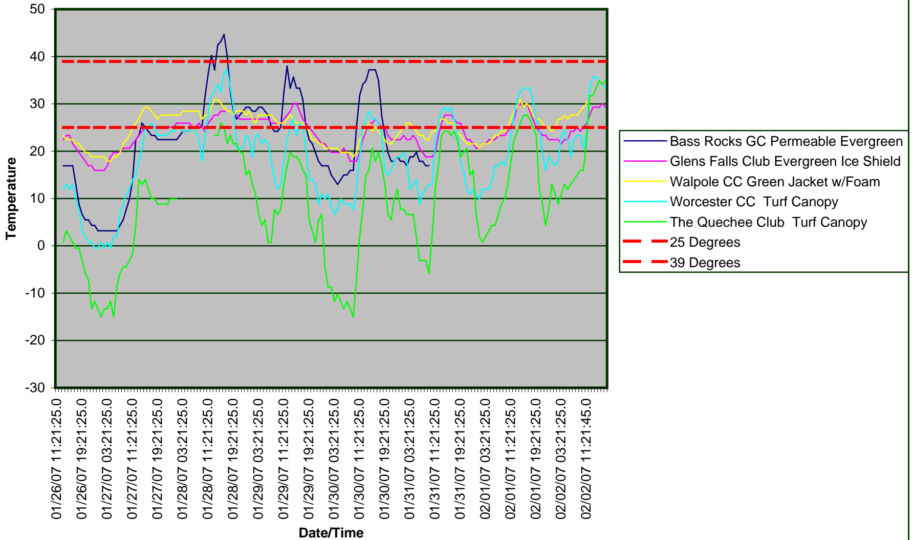
Below Cover/Canopy Temps 1-26-07 to 2-2-07
