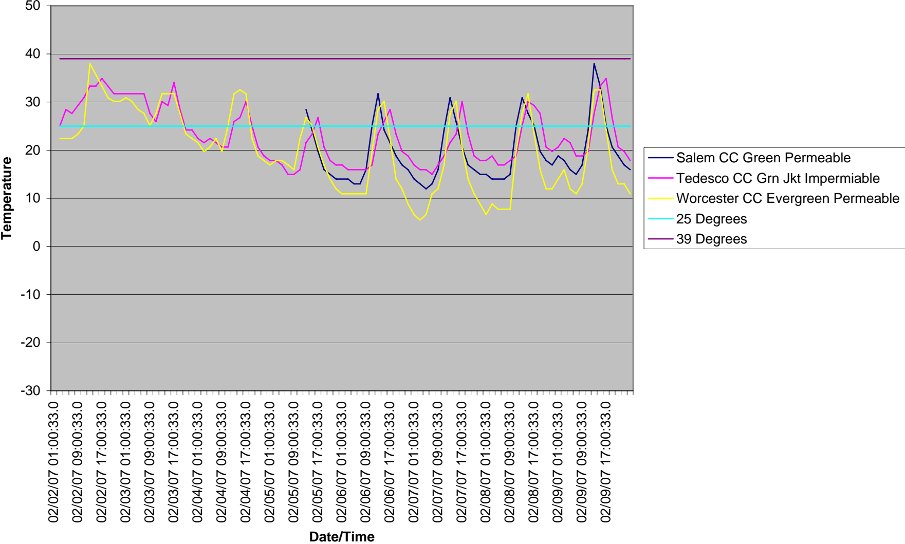
Below Cover/Canopy 2-2-07 to 2-9-07 (2 Hr. Readings)
