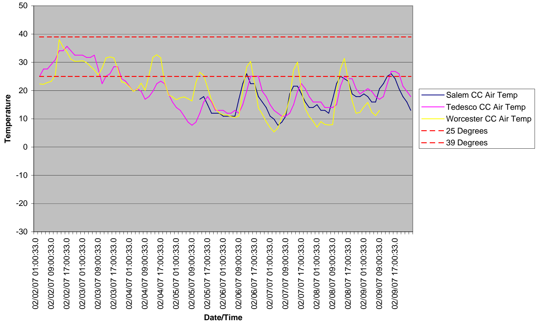
Above Cover/Canopy Temps 2-2-07 to 2-9-07 (2 Hr. Readings)
