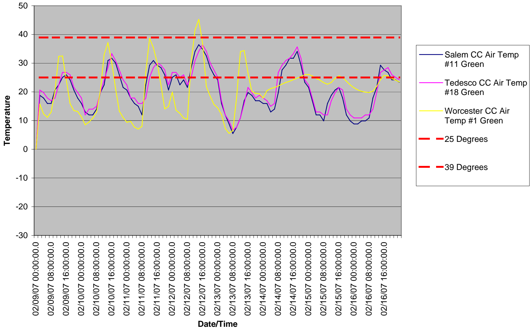
Air Temps 2-9-07 to 2-16-07 (2 Hour Readings)
