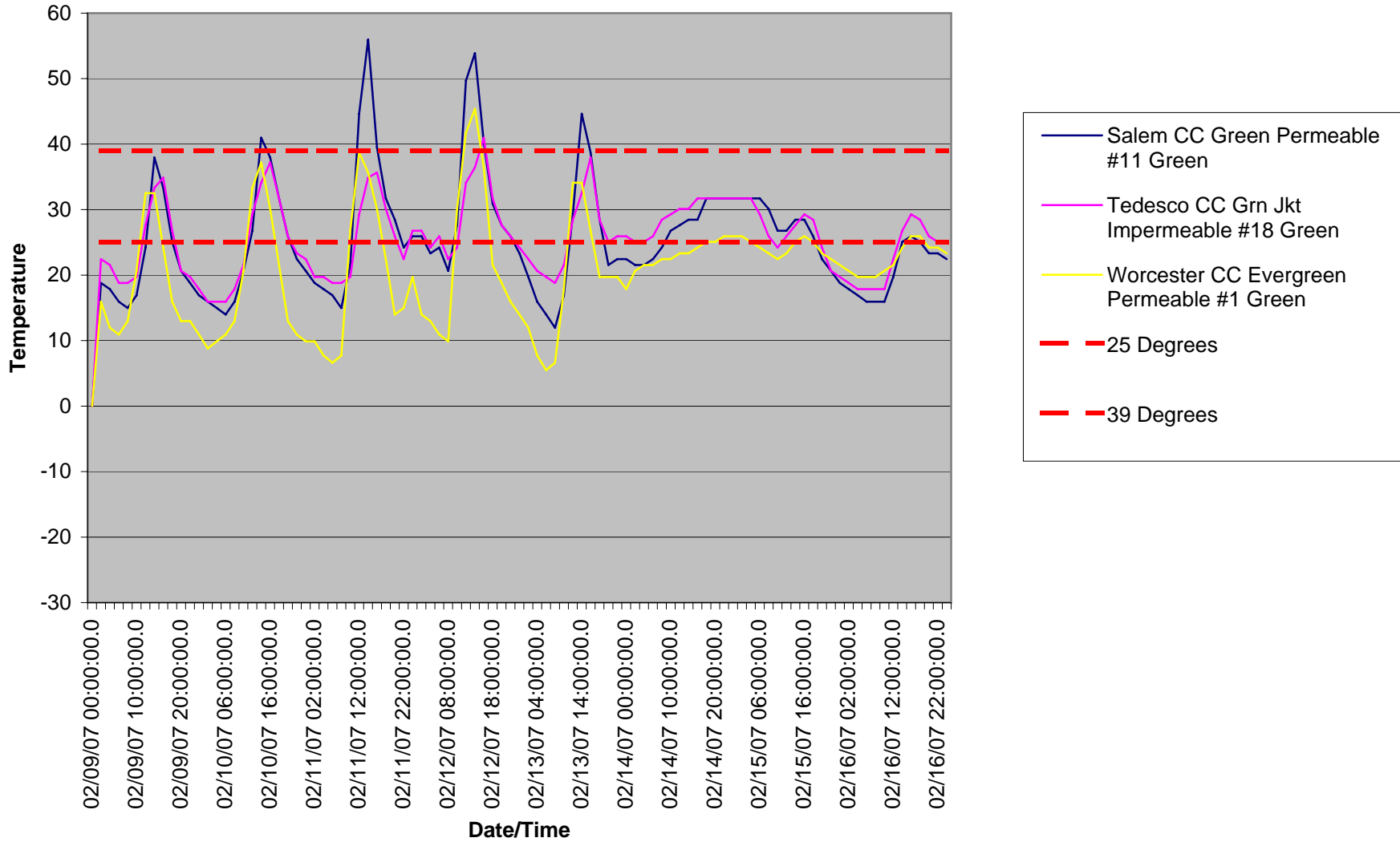
Below Cover Temps 2-9-07 to 2-16-07 (2 Hour Readings)
